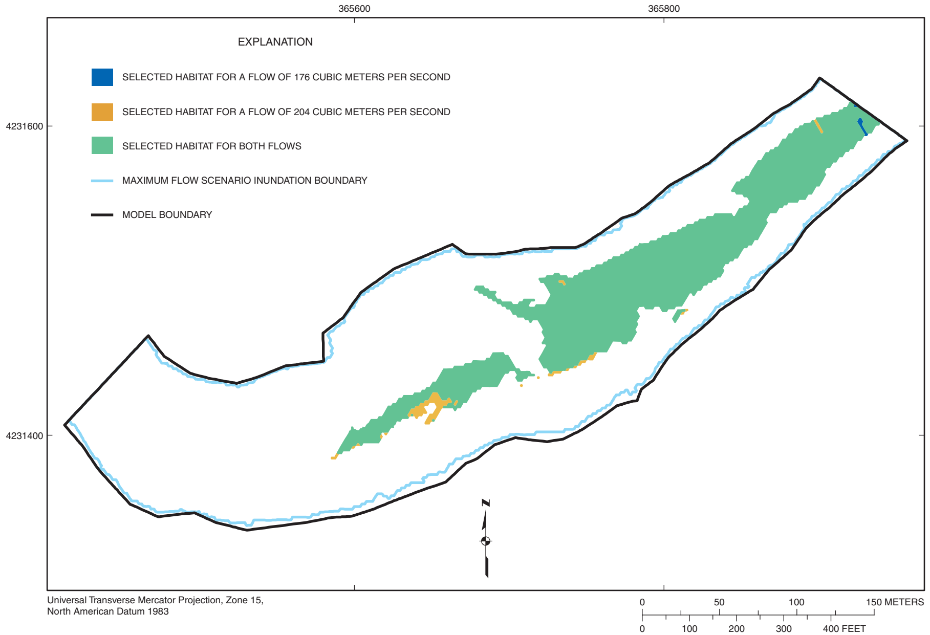
Figure 4-31. Selected habitat area distribution for habitat category 7 (paddlefish) at flows of 176 and 204 cubic meters per second at Marais des Cygnes River site MDC2.
